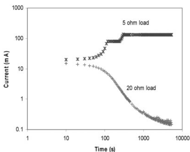
Figure 6b. STR PEM fuel cell startup with different load resistances.
